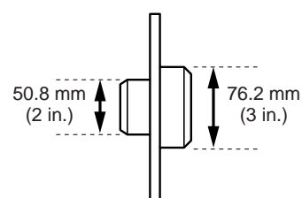
Media flange
